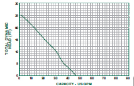
Sump Pump Performance Curve
