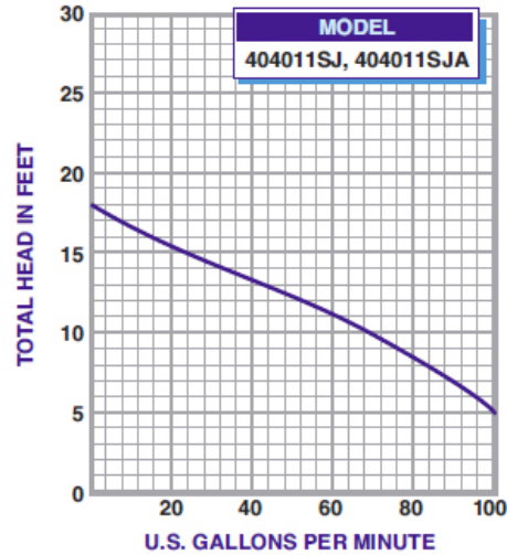
Sewage
